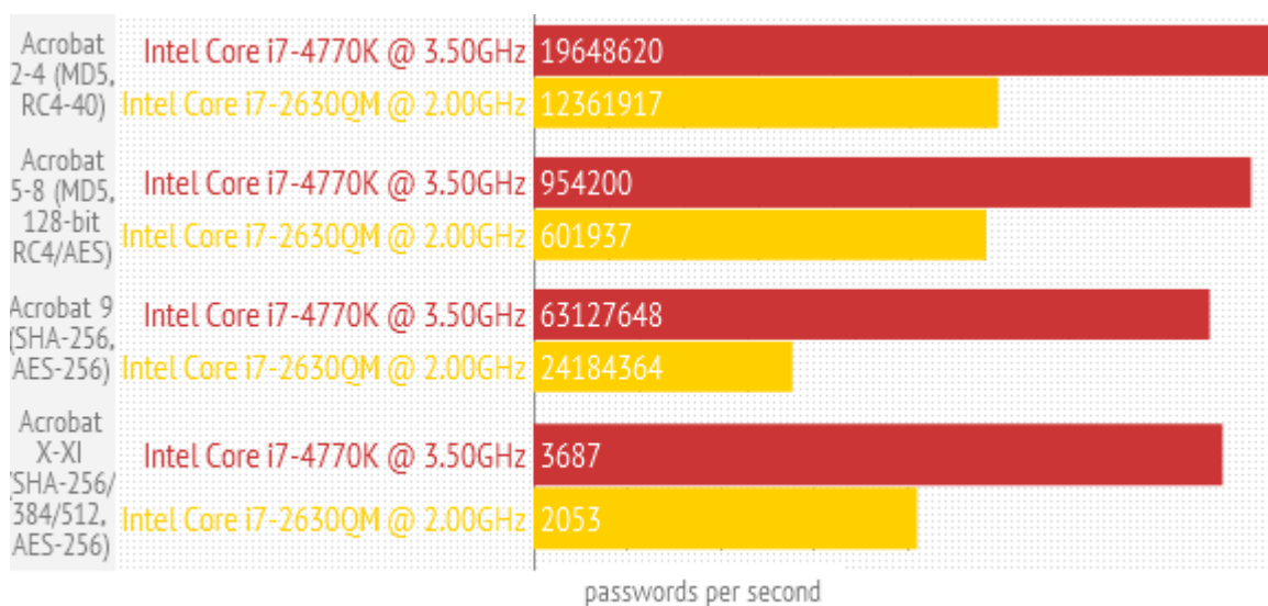
Password Recovery Speed for Adobe PDF created in Adobe Acrobat 2-XI
