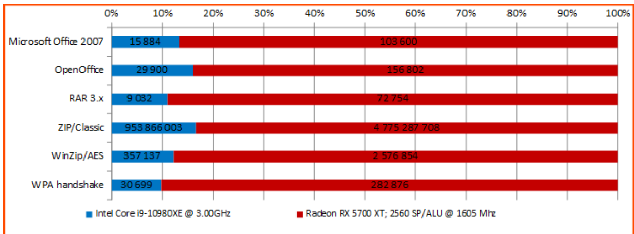
Graphic: Recovery speed difference for CPU and GPU (passwords per second)
